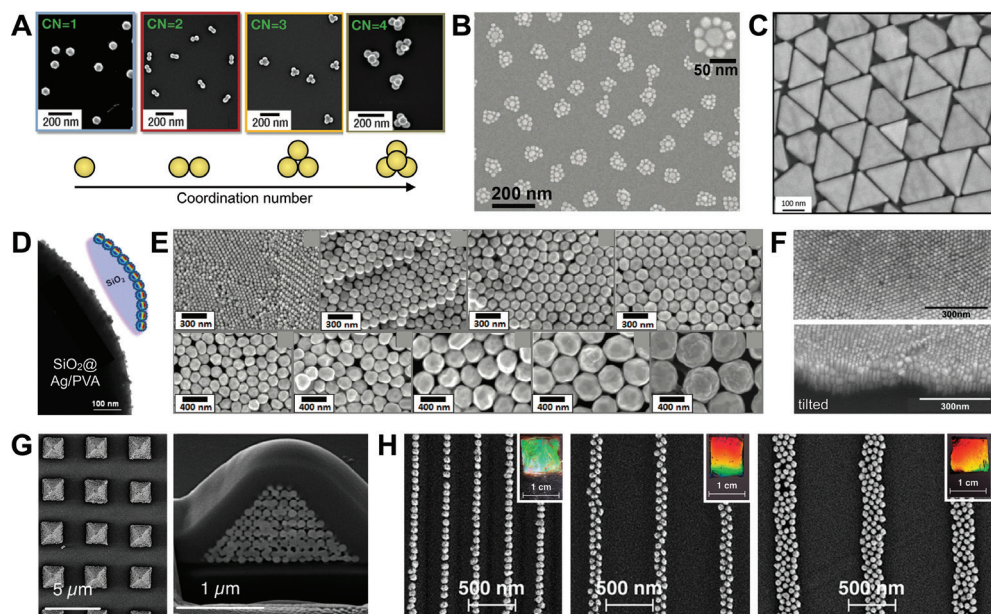
Figure 9. Ordered assemblies designed for high SERS activity. (A) Nanoparticle clusters of discrete coordination numbers. Copyright 2012 Wiley, adapted with permission [109]. (B) DNA-directed 2D core/satellite structures. Copyright 2012 Wiley, adapted with permission [110]. (C) Monolayer of close-packed nanotriangles. Copyright 2017 ACS, adapted with permission [118]. (D) AgNP-decorated silica microparticles. Copyright 2015 ACS, adapted with permission [119]. (E) Patterned supercrystal array of close-packed vertically aligned nanorods. Copyright 2012 Wiley, adapted with permission [124]. (F) Supercrystals of NPs ranging from the nano- to the microscale. Copyright 2012 ACS, adapted with permission [121]. (G) Pattern of pyramidal supercrystal architectures. Copyright 2017 ACS, adapted with permission [126]. (H) Macroscale patterns of quasi-infinite linear NP arrangements. Copyright 2014 ACS, adapted with permission [61].
